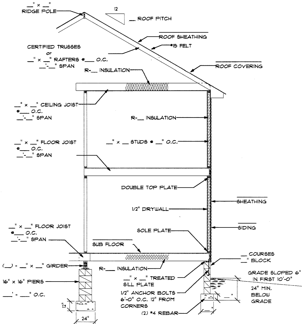
TYPICAL TWO STORY SECTION W/CRAWLSPACE
