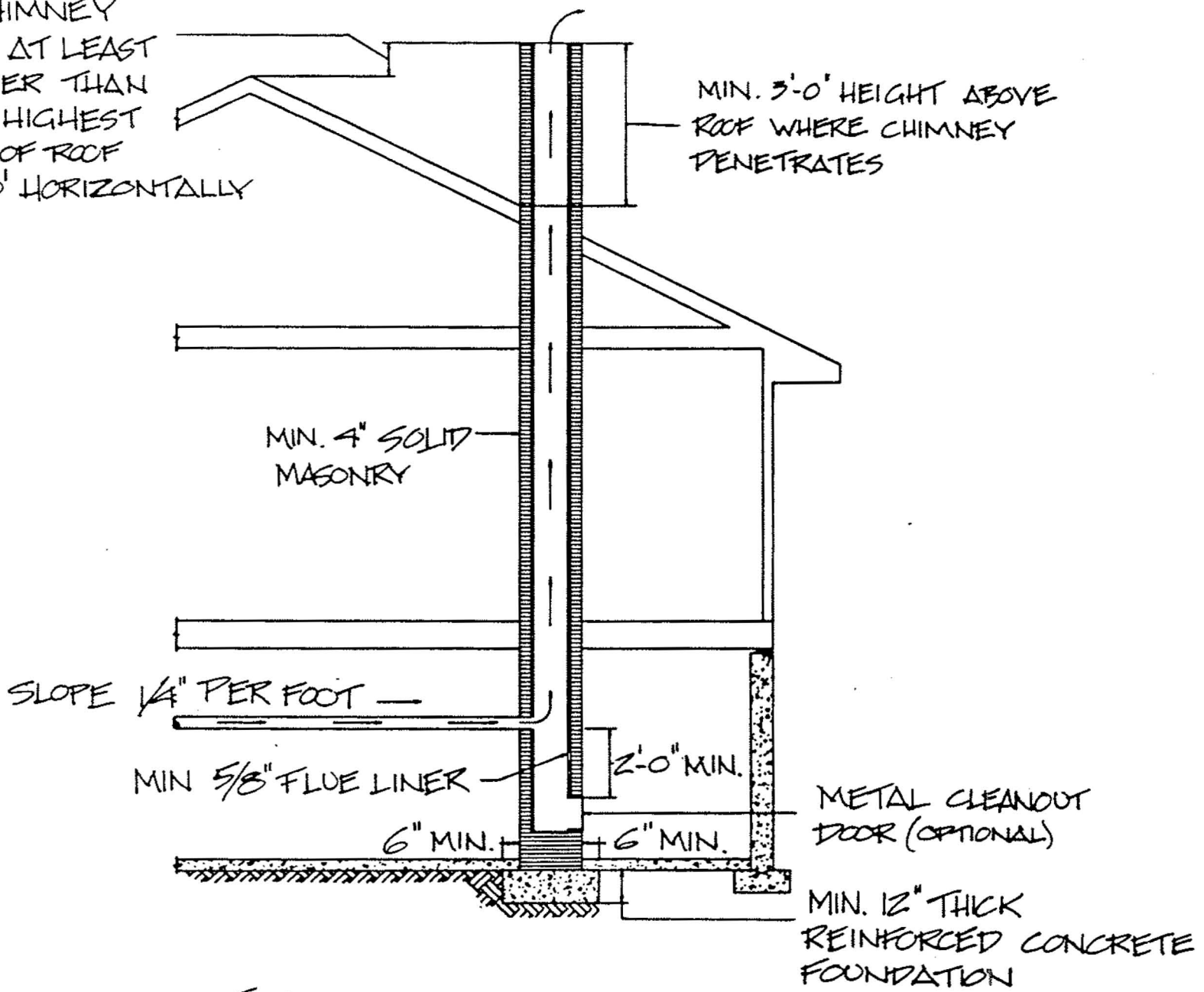
TYPICAL MASONRY CHIMNEY
