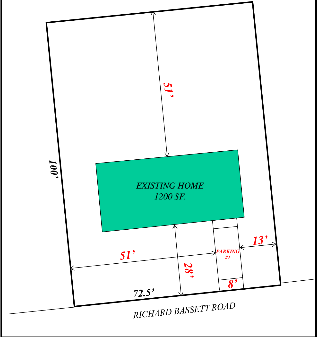
PLOT PLAN
